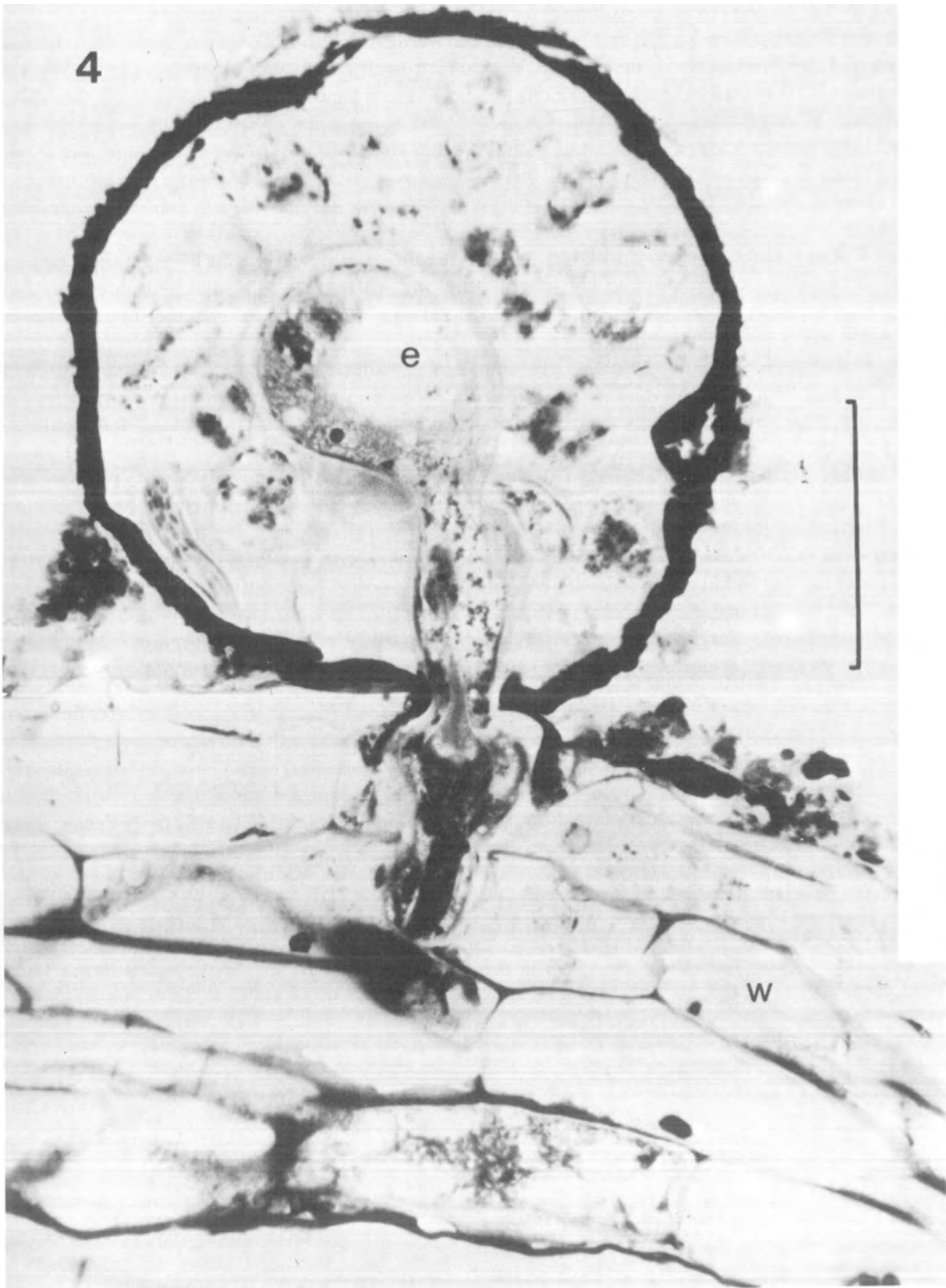
Fig. 4. Balanophora elongata ; the host tissue (w) is penetrated by parasitic cells of the disintegrating endosperm surrounding the embryo (e). Scale corresponds to 0.05 mm
